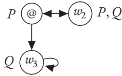
Figure 3.1: A Kripke model. Arrows represent the accessibility relation (here, we have R@w_2, R w_2@, R@w_3, R w_3 w_3 ). The valuation is represented by writing the propositional constants that are true at each world next to the world. Thus, in this model V(P, @)=V(P, w_2)=V(Q, w_2)=V(Q, w_3)=True , and V(Q, @)=V(P, w_3)=False .
